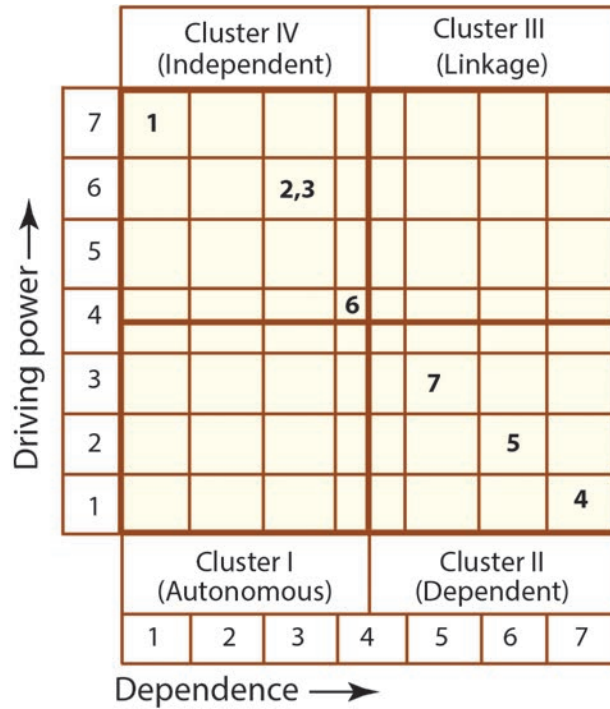
Figure 7.13: MICMAC analysis.
